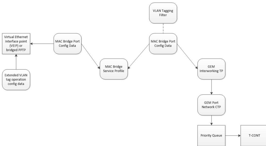
Figure 3 – OMCI Model for Ethernet Traffic Tests
