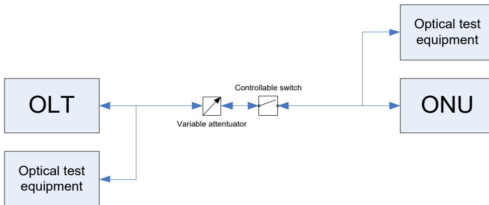
Figure 6 - Test Setup for Intermittent LODS
