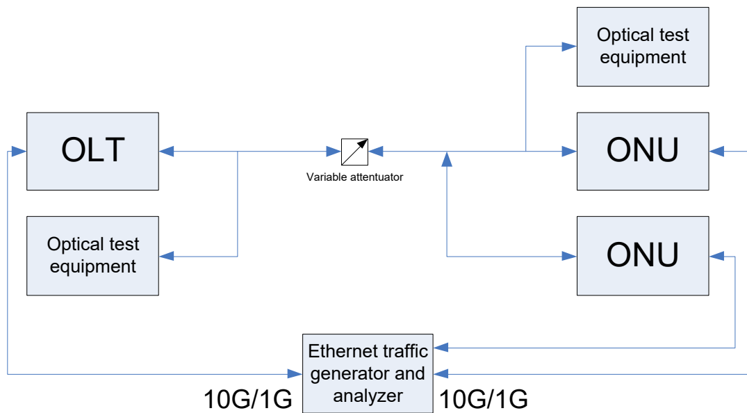
Figure 4 – Multiple ONU Test Setup with Ethernet Traffic
