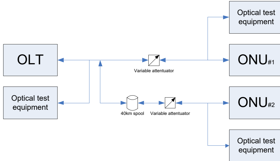
Figure 5 - Test Setup for Differential Reach Test
