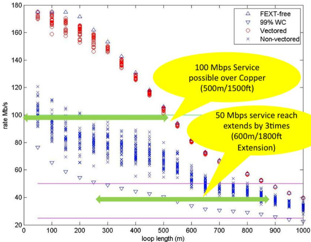
Figure 4: Example VDSL2 performance improvements in a 100 pair cable with vectoring.
