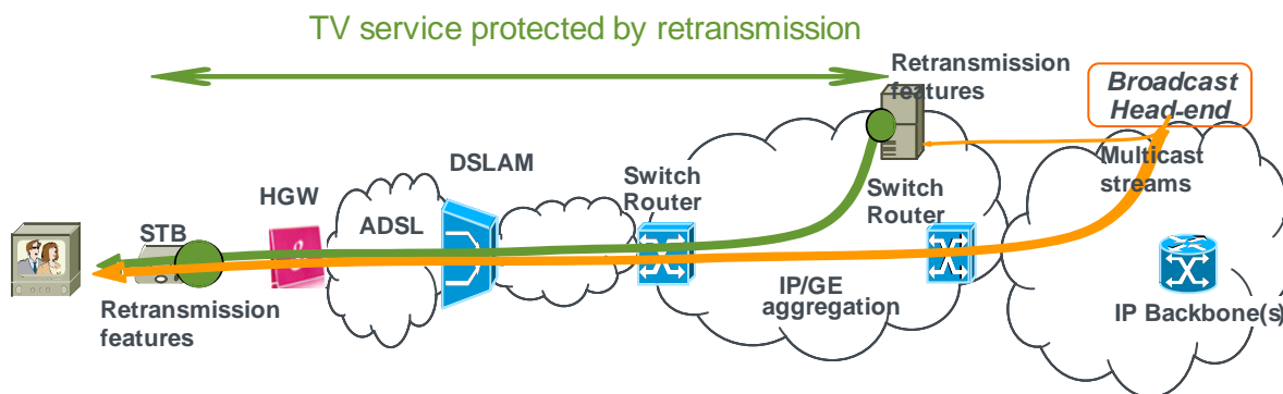
Figure 6: Network architecture for retransmission
