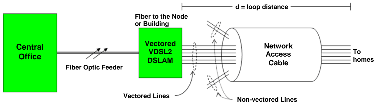
Figure 3: Reference Fiber Fed DSL Network Access Architecture.
