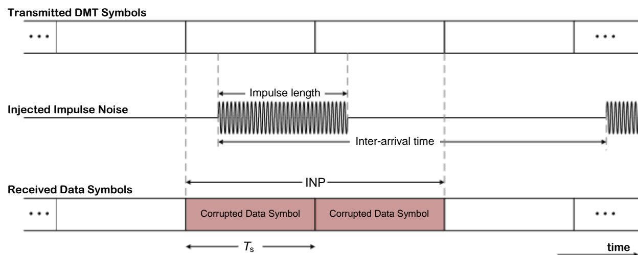
Figure 5: Reference signals demonstrating impact of impulse noise.
